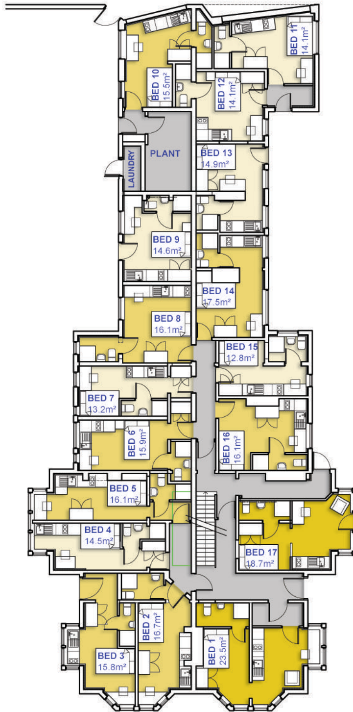
2. Ground Floor Plan
