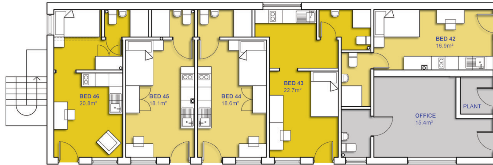
1. Ground Floor Plan
